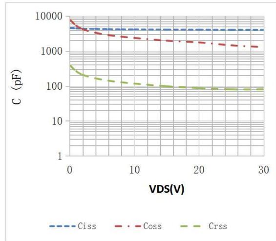
Fig.2 Capacitance Characteristics
