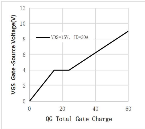
Fig.1 Gate-Charge Characteristics
